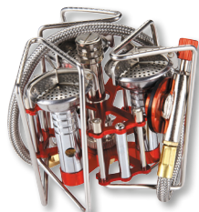
Folded Pan Supports & Legs
